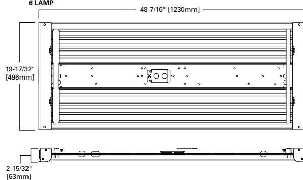
6 LAMP
