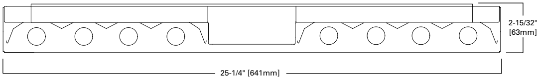
8 LAMP
