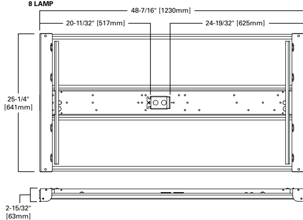
8 LAMP
