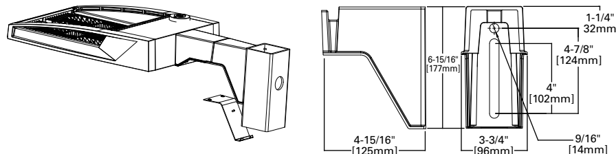
QM Quick Mount Arm (Standard)
