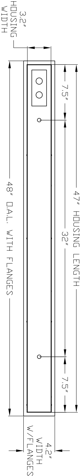
4' INDIVIDUAL FIXTURE (TOP VIEW)
