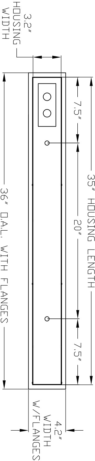
3' INDIVIDUAL FIXTURE (TOP VIEW)
