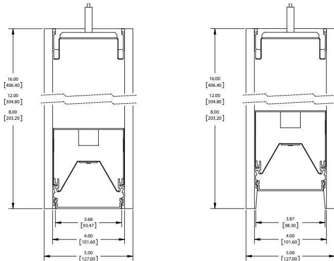
SA4xxDP Flush
