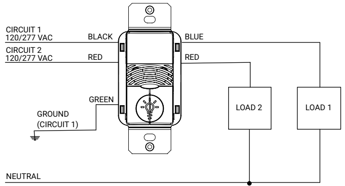
120/277 VAC dual level dual circuit wiring diagram
