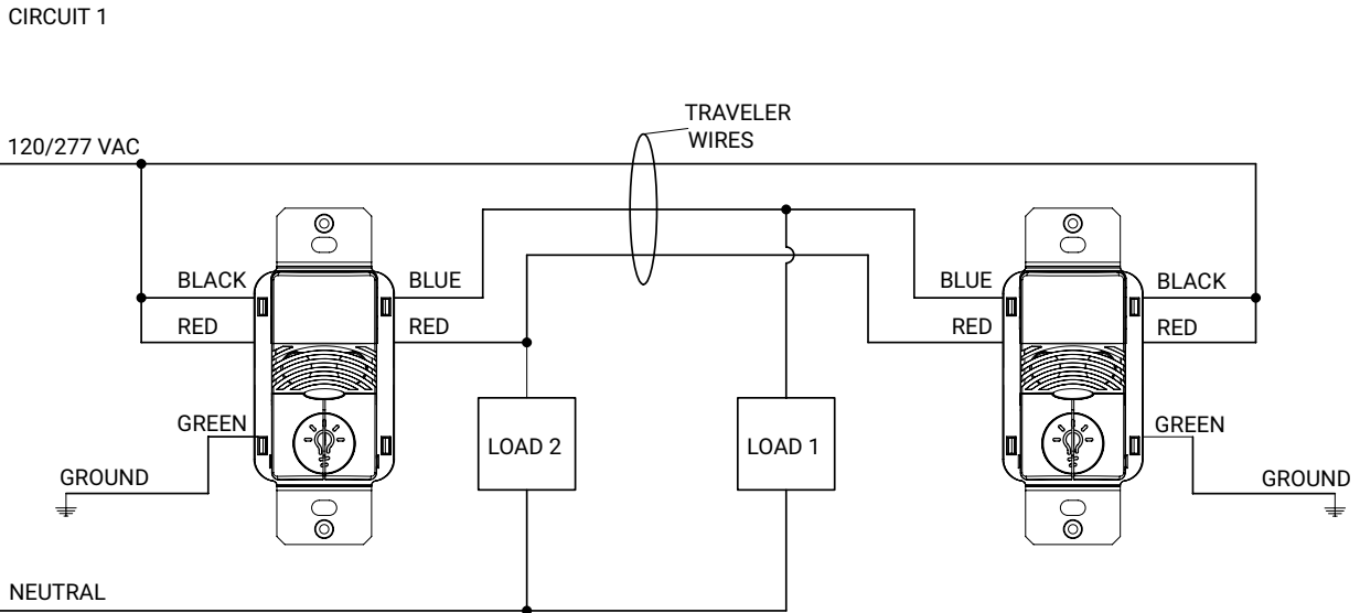
Three-way wiring diagram: Lights will turn OFF automatically when sensor that detected motion last, times out.
