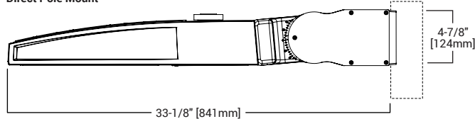
Wall Mount
