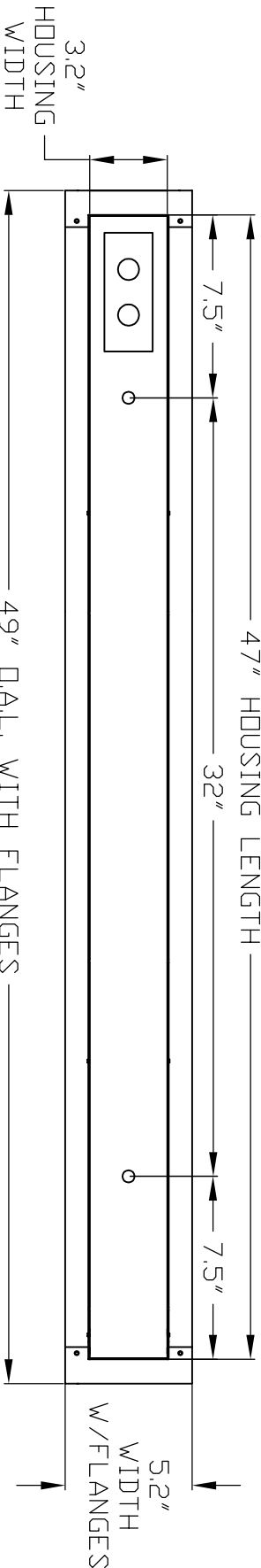
4' INDIVIDUAL FIXTURE (TOP VIEW)
