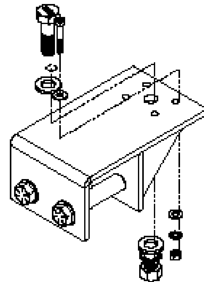
DB3 Diving Board Kit (DVGBRD) with Additional (HRDM34) Mounting Fastener Hardware Kit
