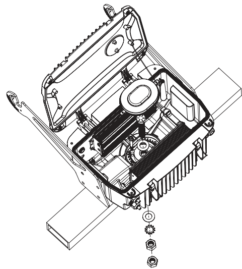
12a Local Yoke Mount
