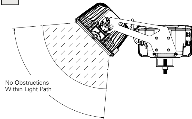
2a Yoke Mount
