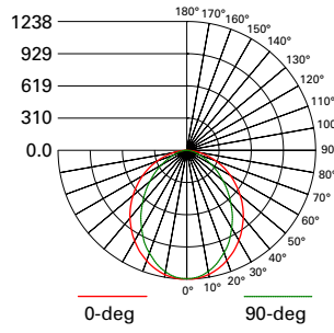
SATIN REGRESSED DIFFUSER
